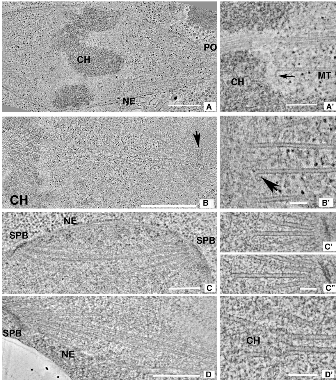
Figure 2. Tomographic slices of the spindles studied here. (A) 10-nm slice from a serial tomogram of a C. reinhardtii metaphase (CrM1, see Fig. S1 for model). Chromosomes (CH), the nuclear envelope (NE), and an opening in the envelope (PO) through which MTs project toward the spindle pole are evident. (A') 4-nm slice through a different metaphase spindle (CrM2 in Fig. S1). One MT ends near a chromosome (a KMT) but others continue. The arrow indicates a flared PF. (B) 10-nm slice from a serial tomogram of a one-cell embryo of C. elegans . Chromosomes (CH) are evident, and a centriole (arrow) marks the spindle pole. (B') 4-nm slice through the chromosome–MT interface of a different C. elegans metaphase (CeM in Fig. S2). Chromatin, at left, is separated by a fibrous zone from the KMTs with flaring plus ends. No outer plate is seen. (C) 10-nm slice from a tomogram of a metaphase budding yeast (ScM1, Fig. S3); SPB, spindle pole body; NE, nuclear envelope. (C' and C'') Two 4-nm slices from a prometaphase budding yeast (SpPM1); slender filaments connect the capped MT minus ends with the spindle pole. (D) 10-nm slice from a prometaphase fission yeast (SpPM in Fig. S4 C); SPB and the NE are evident, but chromosomes are not. (D') A 4-nm slice from the same cell. Some MTs end in pairs where the texture of nucleoplasm is different (CH). Such MTs have been interpreted as KMTs. Bars: (A) 0.5 \mu\text{m} ; (A') 200 nm; (B) 1 \mu\text{m} ; (B') 100 nm; (C) 0.5 \mu\text{m} ; (C' and C'') 100 nm; (D) 0.5 \mu\text{m} ; (D') 100 nm.
